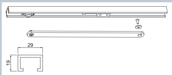
Montage Gleitschiene IS 30 MFA
